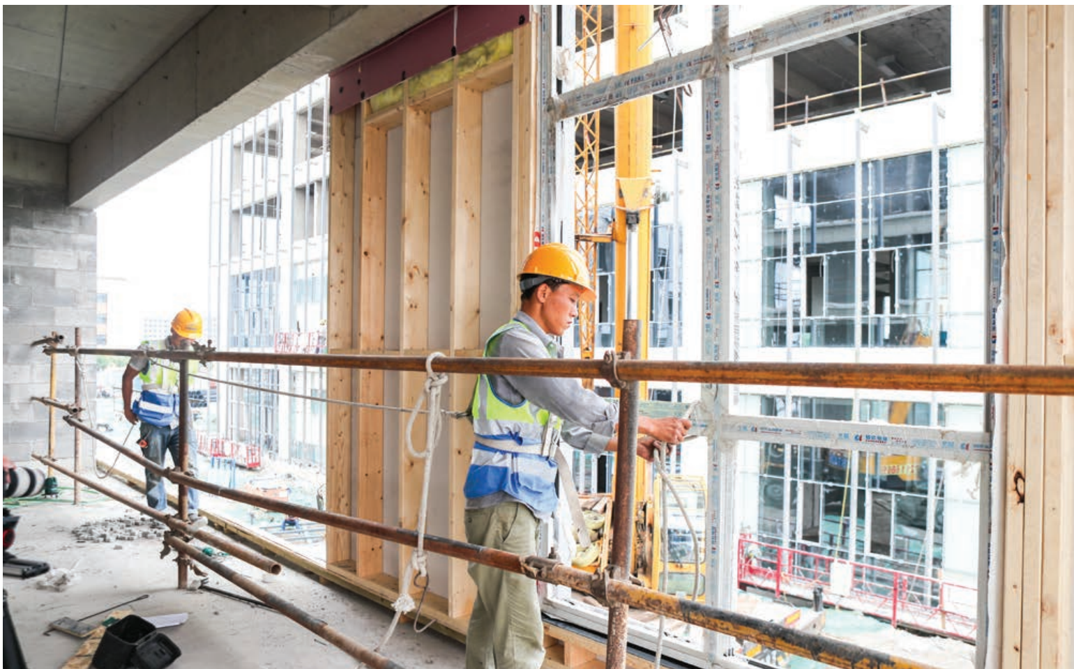
C-Mars Office Project—installing the prefabricated wood wall | Photo: Canada Wood China
