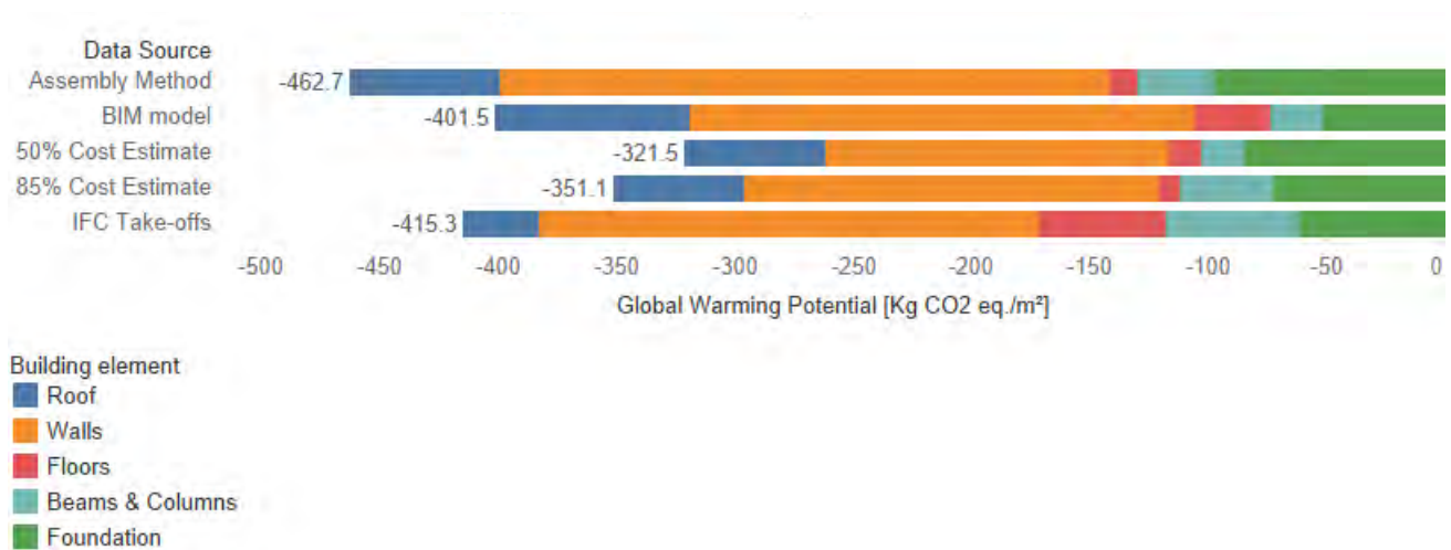
Figure 22: Comparison of GWP (embodied carbon) impacts of the CEC building estimated through WBLCA using different data sources and BoM calculation methods, and broken down by building element.
